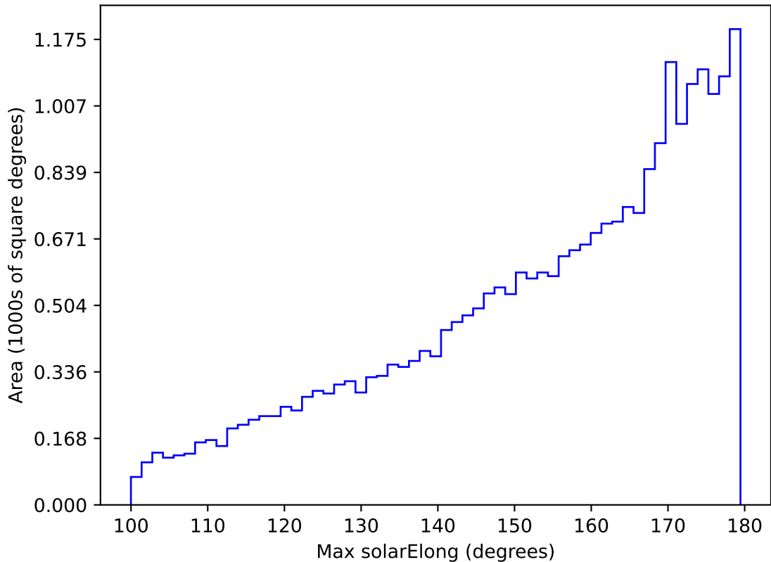
weather_cloudso16v3.4_10yrs All sky r band: Max solarElong
