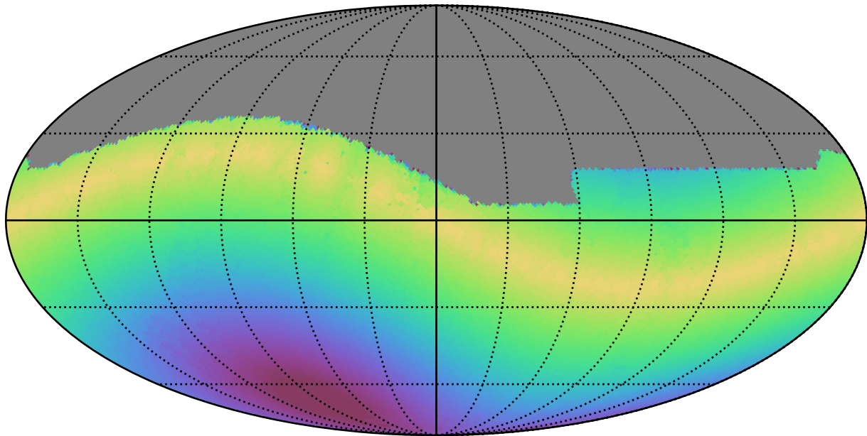
weather_cloudso16v3.4_10yrs All sky g band: Max solarElong
