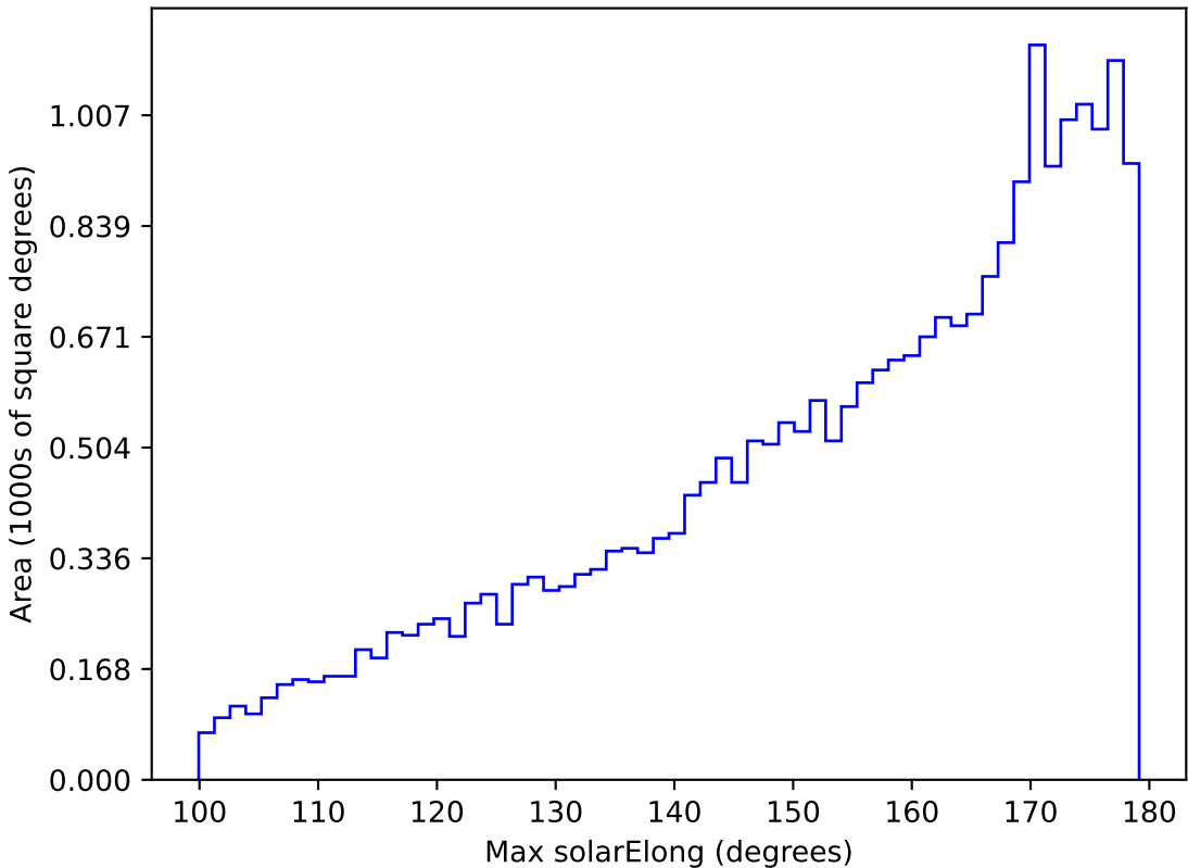
weather_cloudso16v3.4_10yrs All sky g band: Max solarElong
