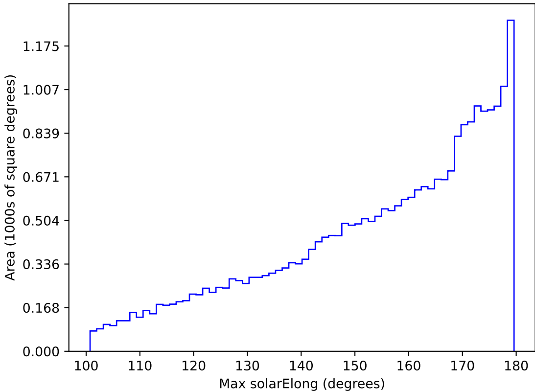
weather_cloudso16v3.4_10yrs All sky all bands: Max solarElong
