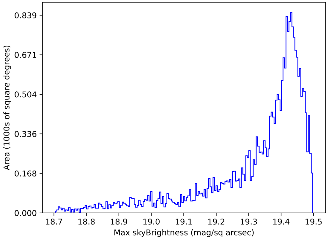
weather_cloudso16v3.4_10yrs Yr 1 z band: Max skyBrightness
