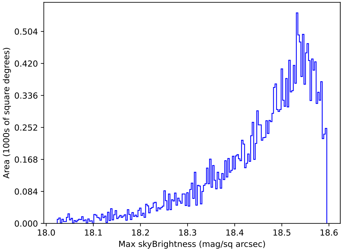
weather_cloudso16v3.4_10yrs Yr 1 y band: Max skyBrightness
