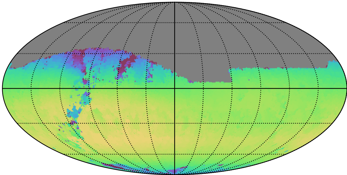
weather_cloudso16v3.4_10yrs Yr 1 i band: Max skyBrightness
