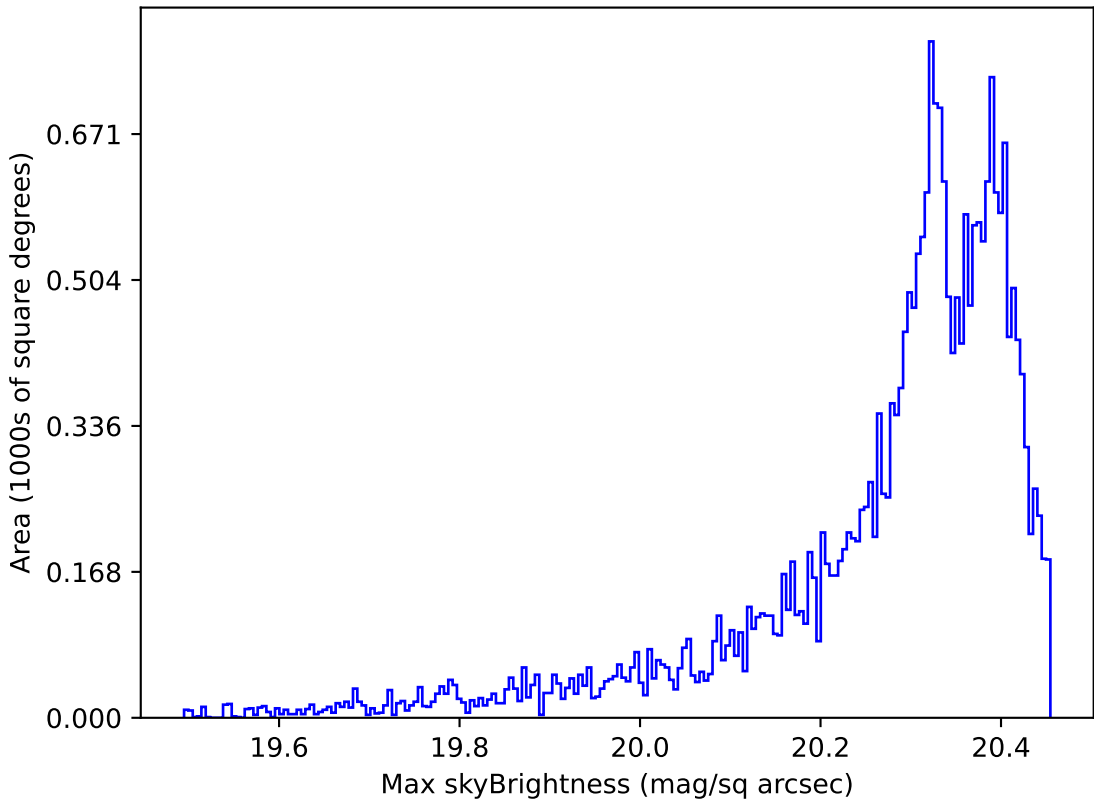
weather_cloudso16v3.4_10yrs Yr 1 i band: Max skyBrightness
