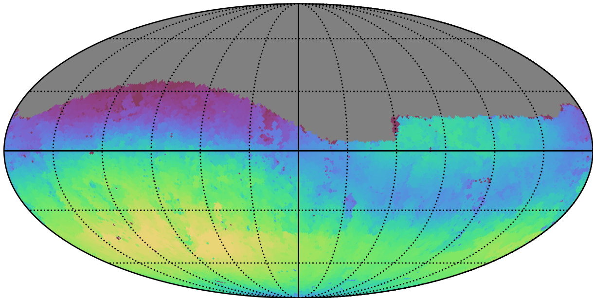
weather_cloudso16v3.4_10yrs Yr 1 g band: Max skyBrightness
