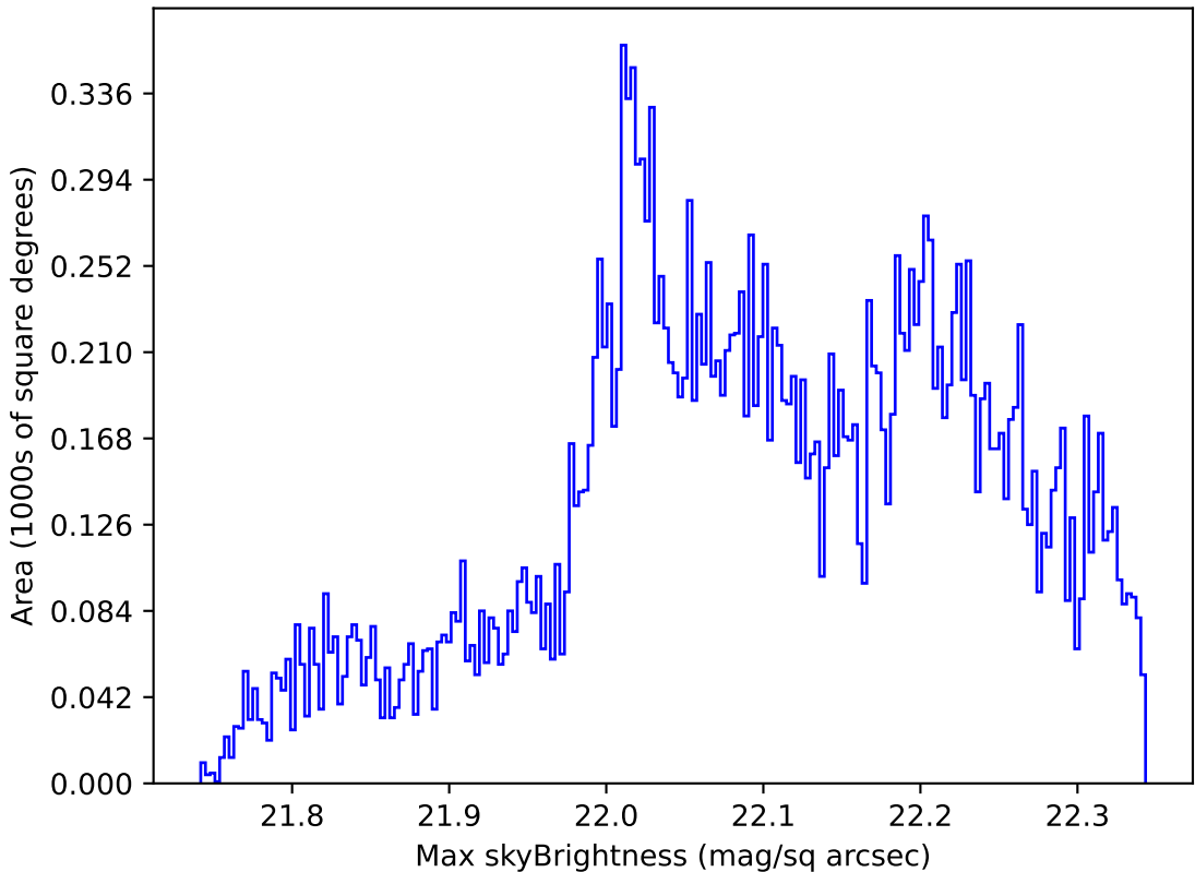
weather_cloudso16v3.4_10yrs Yr 1 g band: Max skyBrightness
