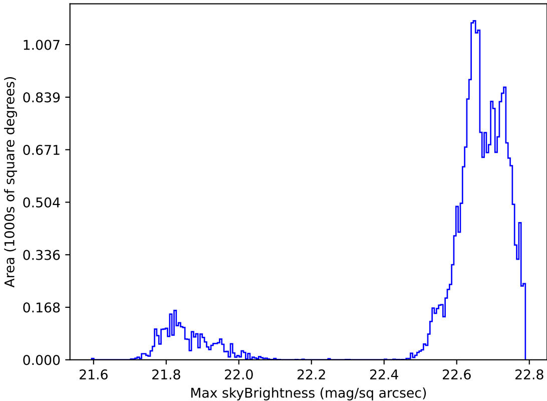
weather_cloudso16v3.4_10yrs Yr 1 all bands: Max skyBrightness
