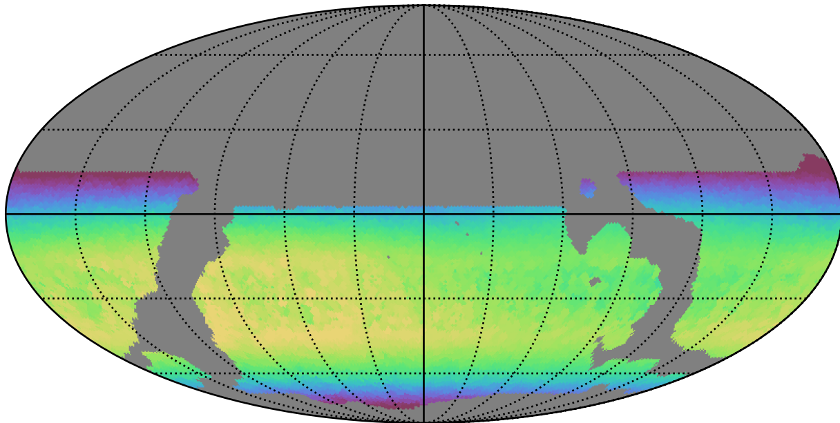
weather_cloudso16v3.4_10yrs WFD z band: Max skyBrightness
