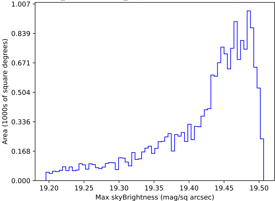
weather_cloudso16v3.4_10yrs WFD z band: Max skyBrightness
