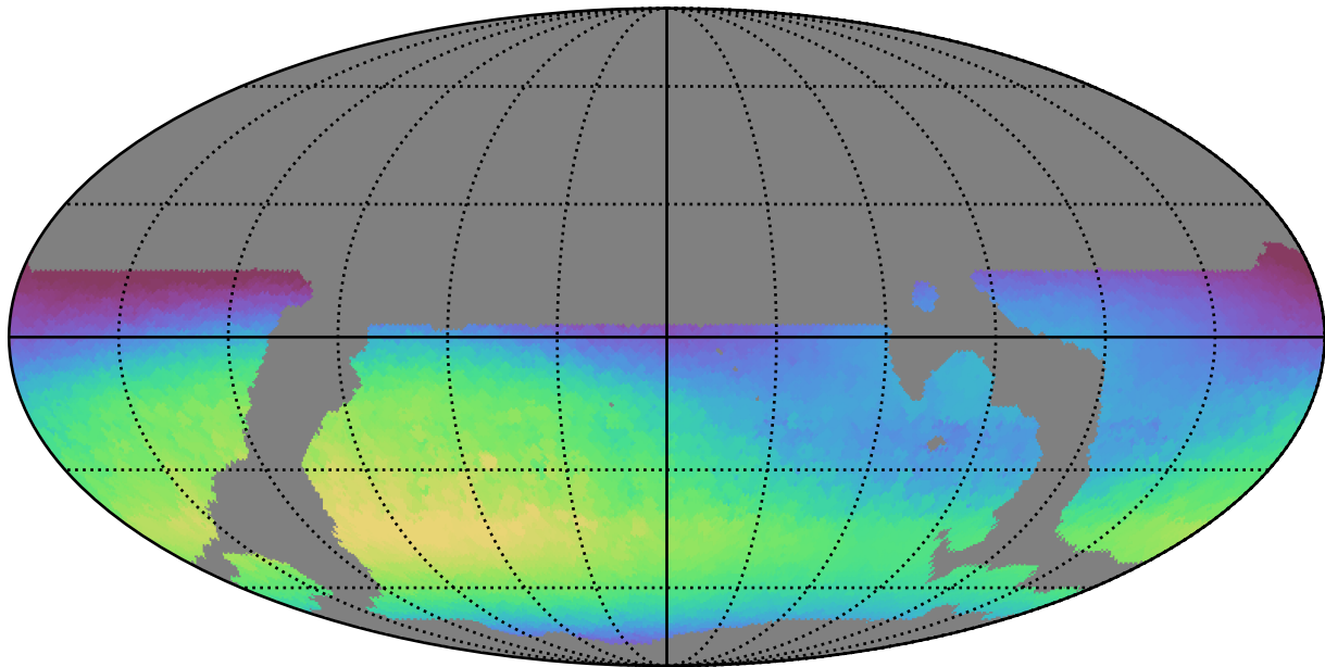
weather_cloudso16v3.4_10yrs WFD u band: Max skyBrightness
