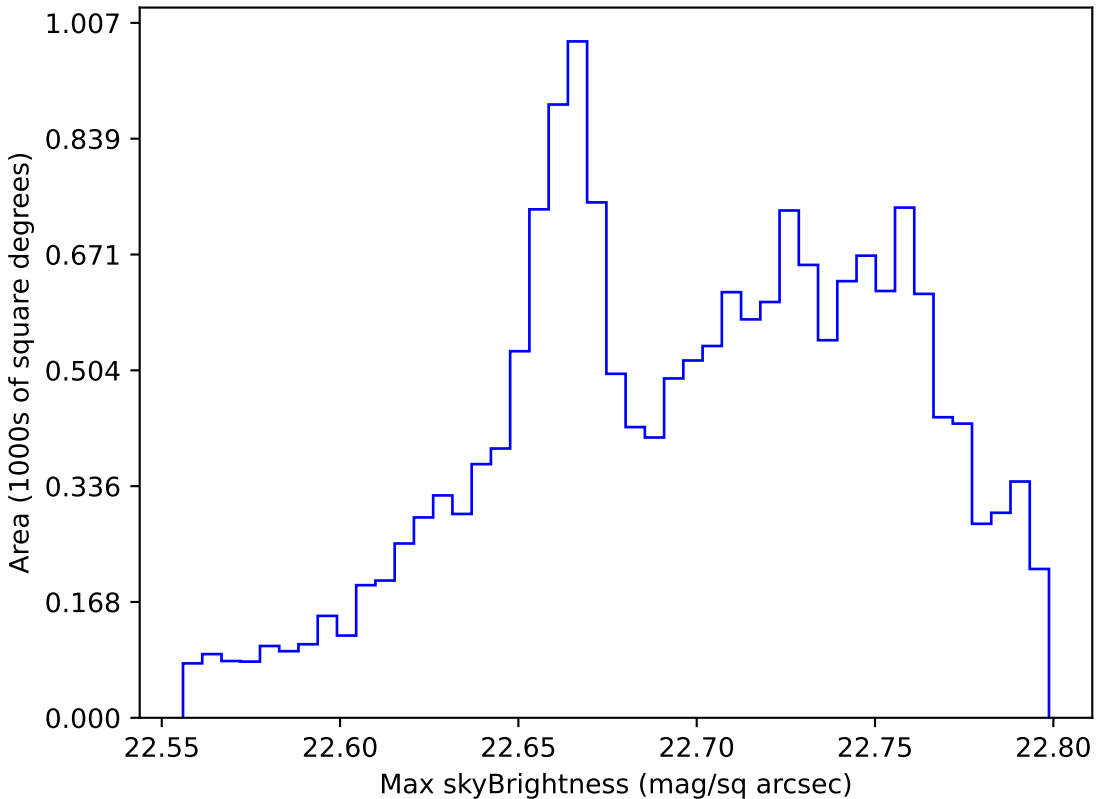
weather_cloudso16v3.4_10yrs WFD u band: Max skyBrightness
