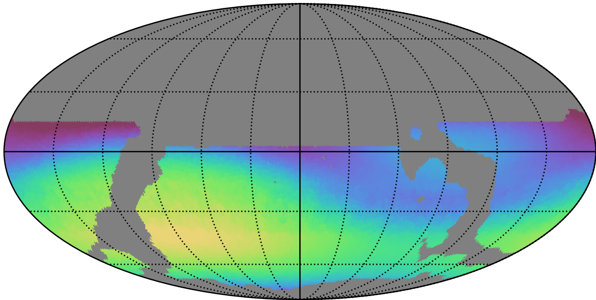
weather_cloudso16v3.4_10yrs WFD r band: Max skyBrightness
