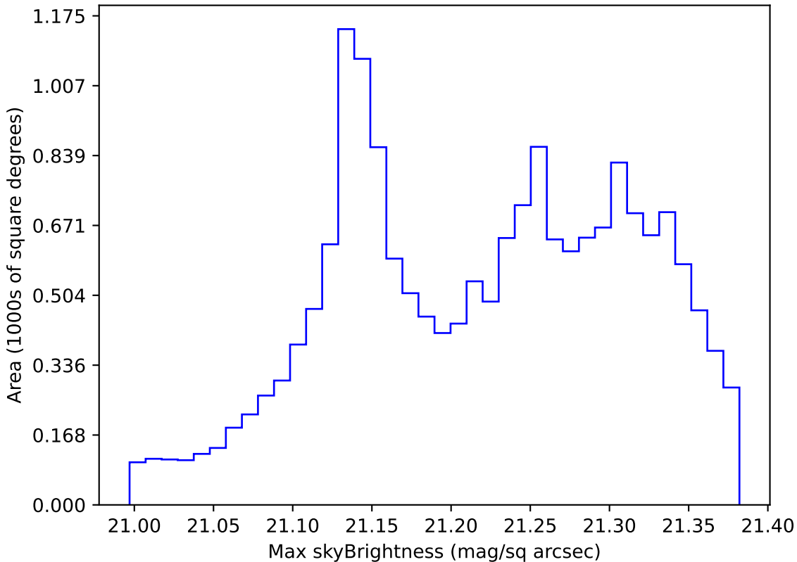
weather_cloudso16v3.4_10yrs WFD r band: Max skyBrightness
