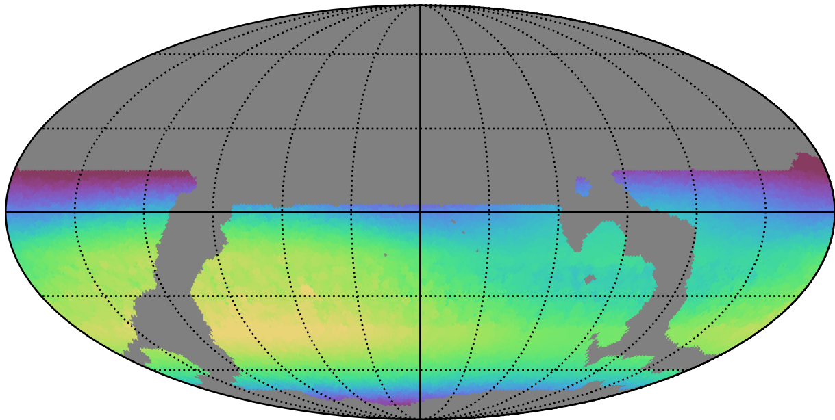
weather_cloudso16v3.4_10yrs WFD i band: Max skyBrightness
