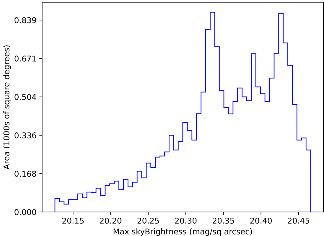
weather_cloudso16v3.4_10yrs WFD i band: Max skyBrightness
