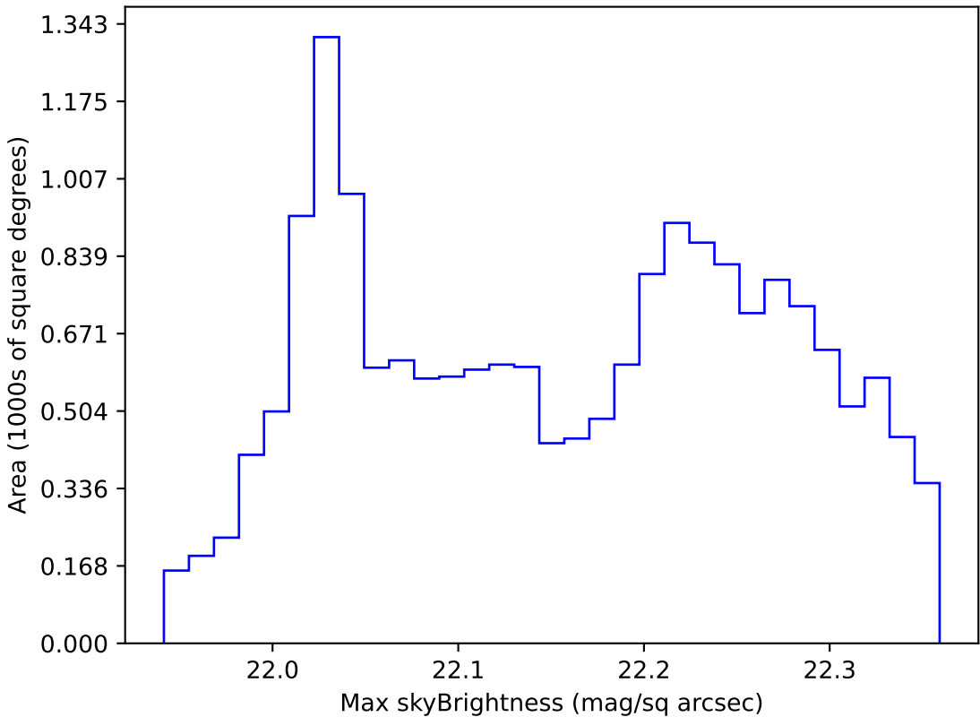
weather_cloudso16v3.4_10yrs WFD g band: Max skyBrightness
