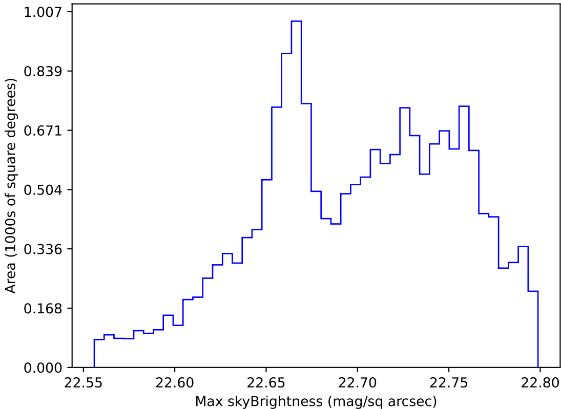
weather_cloudso16v3.4_10yrs WFD all bands: Max skyBrightness
