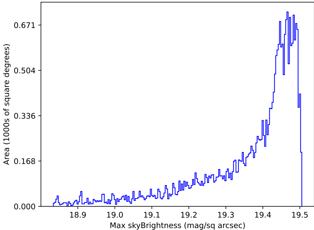
weather_cloudso16v3.4_10yrs All sky z band: Max skyBrightness
