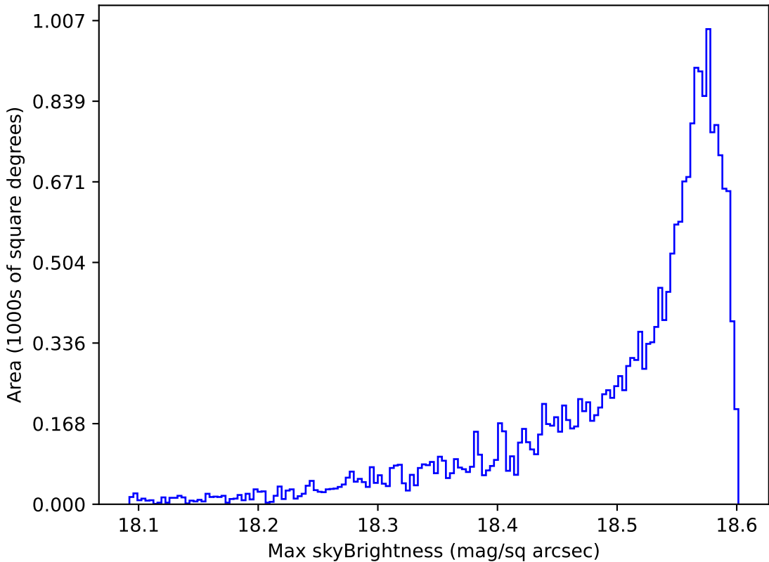
weather_cloudso16v3.4_10yrs All sky y band: Max skyBrightness
