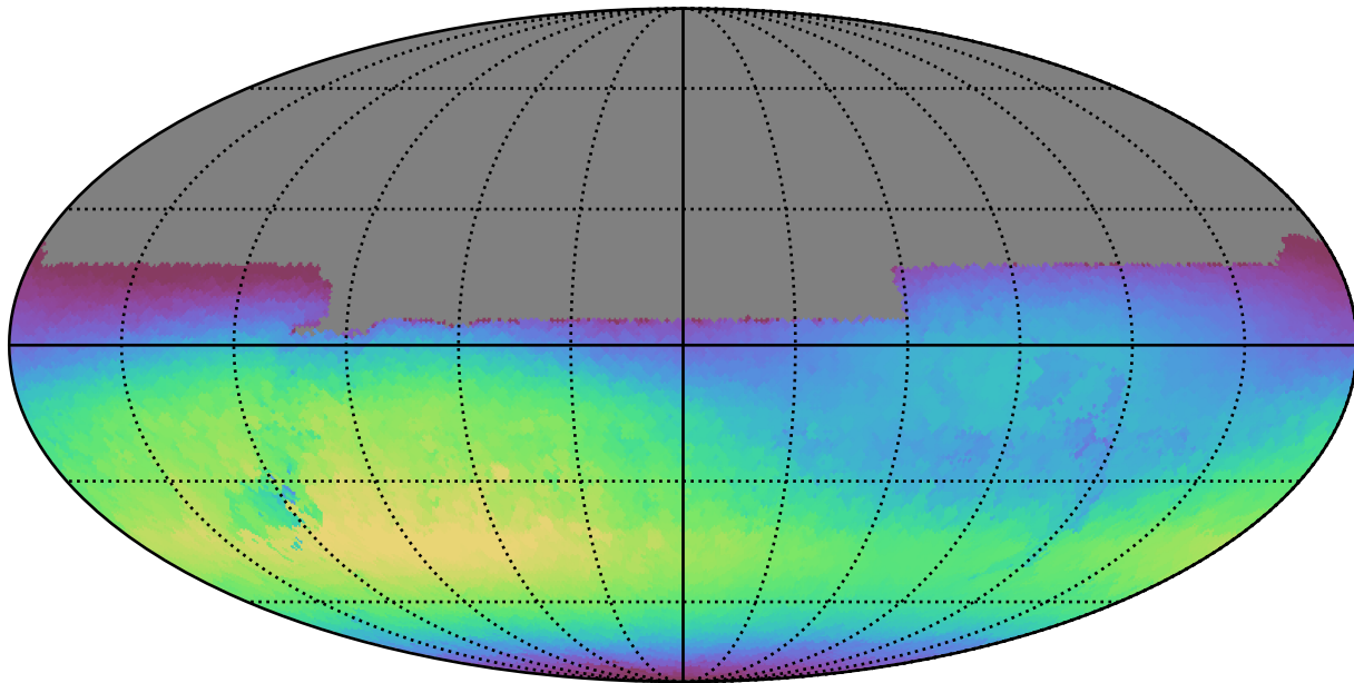
weather_cloudso16v3.4_10yrs All sky u band: Max skyBrightness
