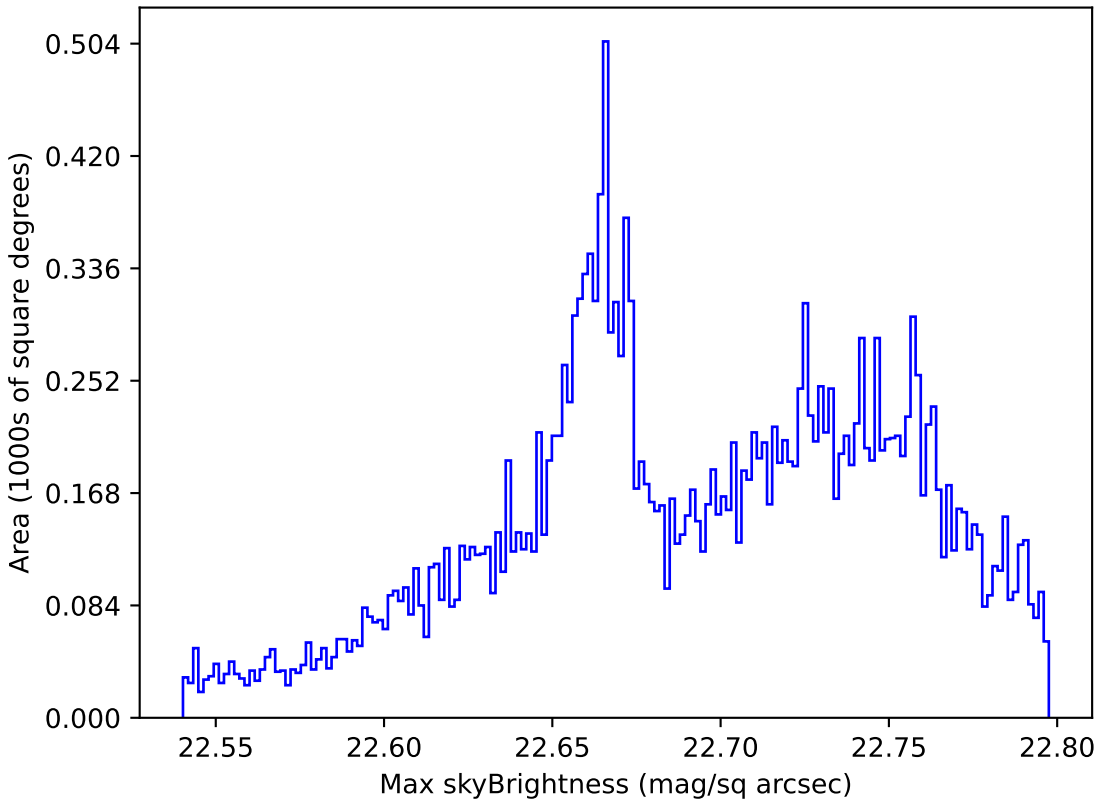
weather_cloudso16v3.4_10yrs All sky u band: Max skyBrightness
