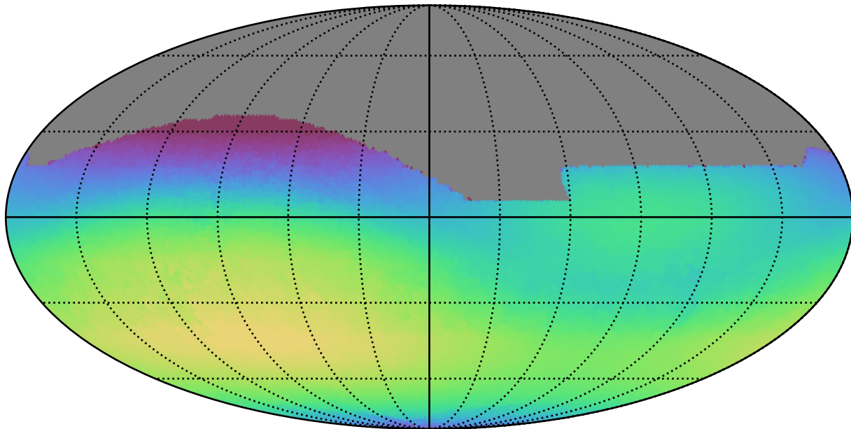
weather_cloudso16v3.4_10yrs All sky r band: Max skyBrightness
