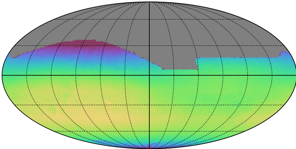
weather_cloudso16v3.4_10yrs All sky i band: Max skyBrightness
