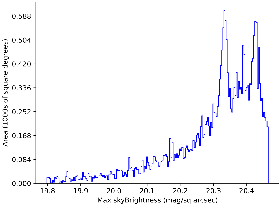
weather_cloudso16v3.4_10yrs All sky i band: Max skyBrightness
