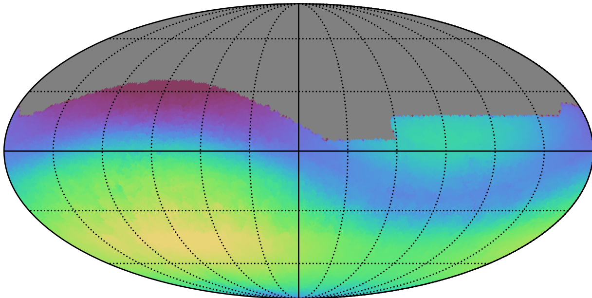
weather_cloudso16v3.4_10yrs All sky g band: Max skyBrightness
