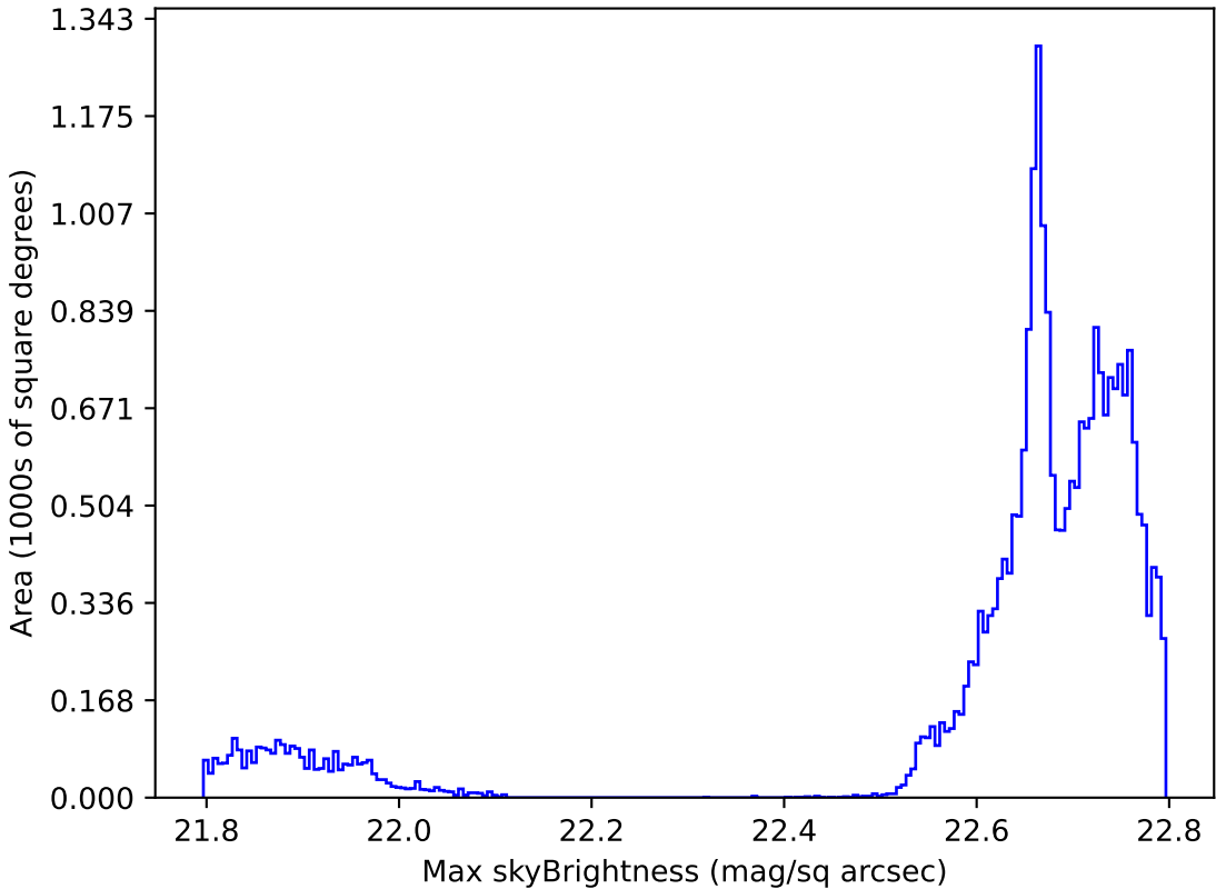
weather_cloudso16v3.4_10yrs All sky all bands: Max skyBrightness
