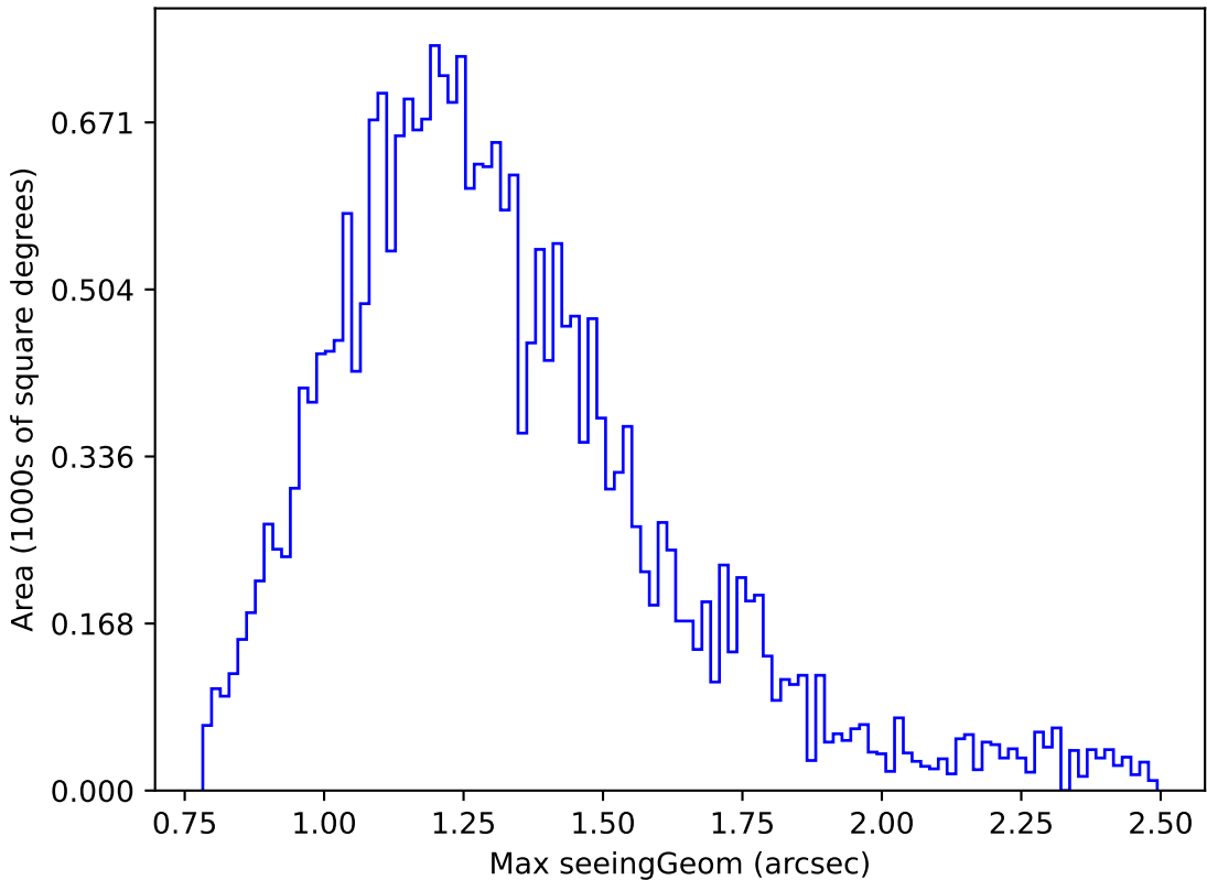
weather_cloudso16v3.4_10yrs Yr 1 z band: Max seeingGeom
