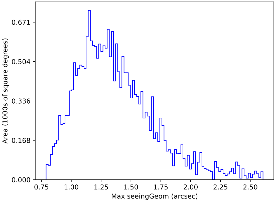
weather_cloudso16v3.4_10yrs Yr 1 u band: Max seeingGeom
