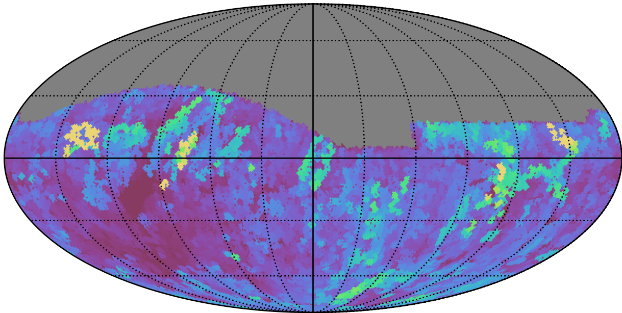
weather_cloudso16v3.4_10yrs Yr 1 r band: Max seeingGeom
