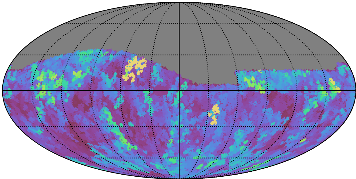
weather_cloudso16v3.4_10yrs Yr 1 i band: Max seeingGeom
