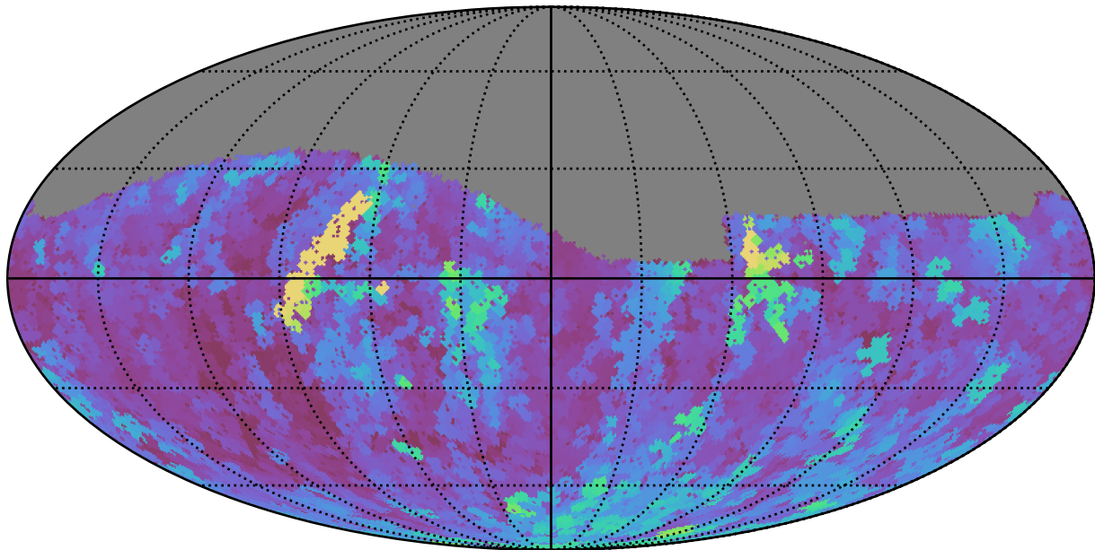
weather_cloudso16v3.4_10yrs Yr 1 g band: Max seeingGeom
