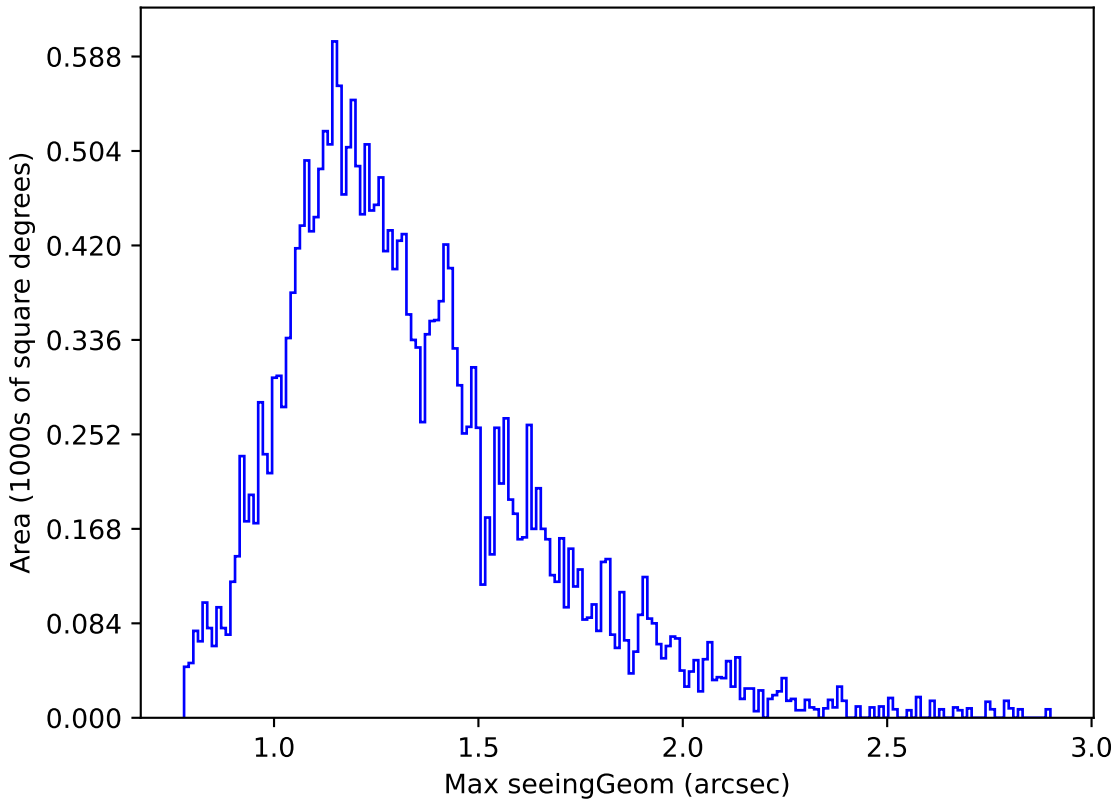
weather_cloudso16v3.4_10yrs Yr 1 g band: Max seeingGeom
