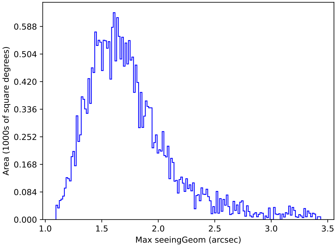
weather_cloudso16v3.4_10yrs Yr 1 all bands: Max seeingGeom
