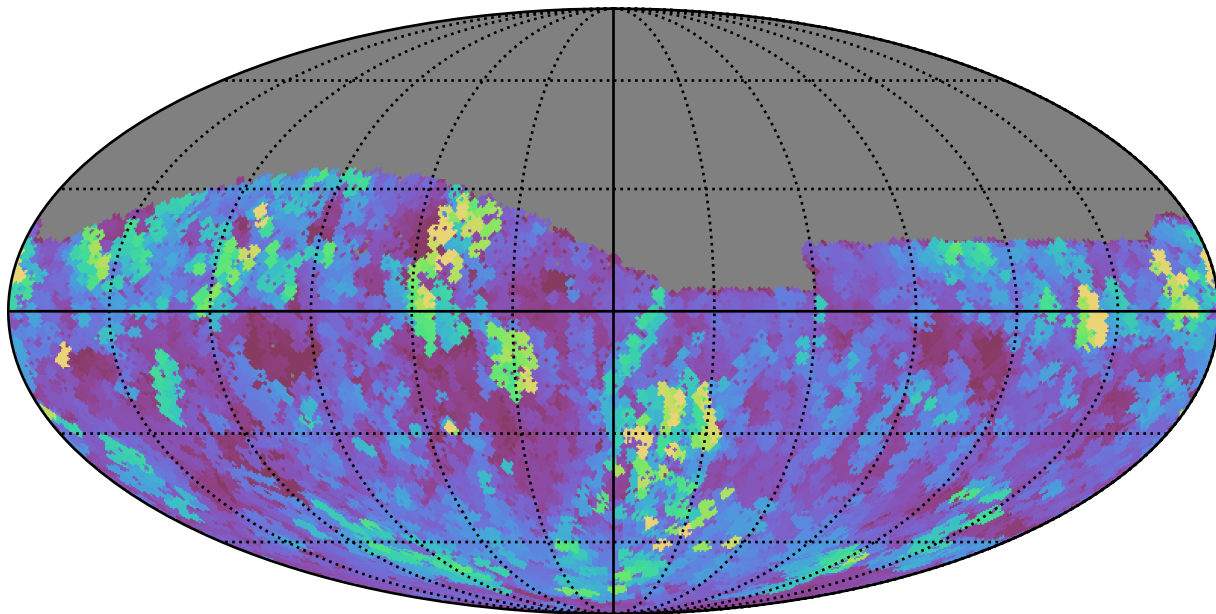
weather_cloudso16v3.4_10yrs Yr 1 z band: Max seeingEff
