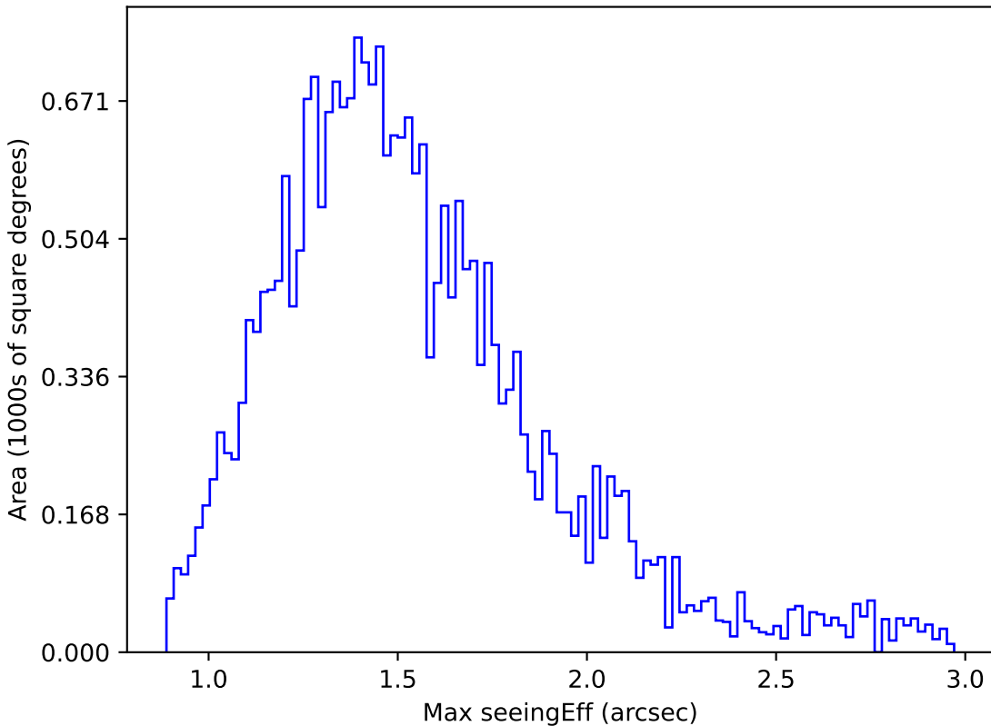
weather_cloudso16v3.4_10yrs Yr 1 z band: Max seeingEff
