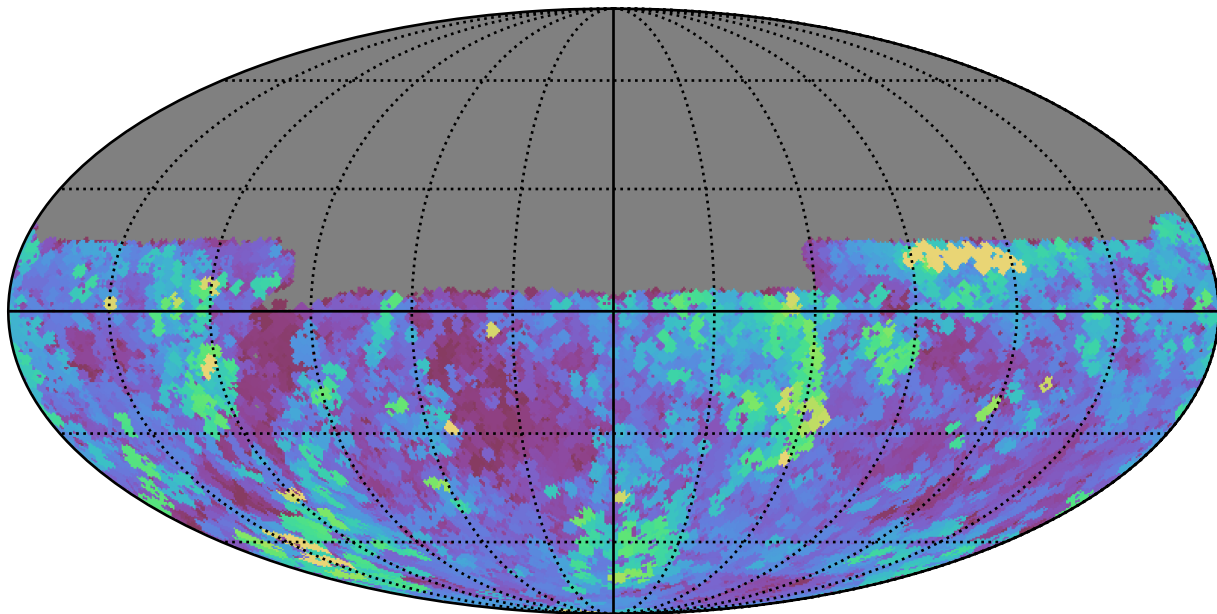
weather_cloudso16v3.4_10yrs Yr 1 y band: Max seeingEff
