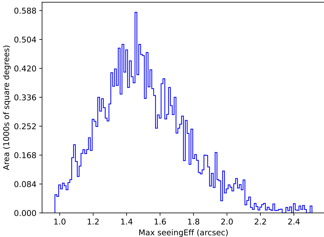
weather_cloudso16v3.4_10yrs Yr 1 y band: Max seeingEff
