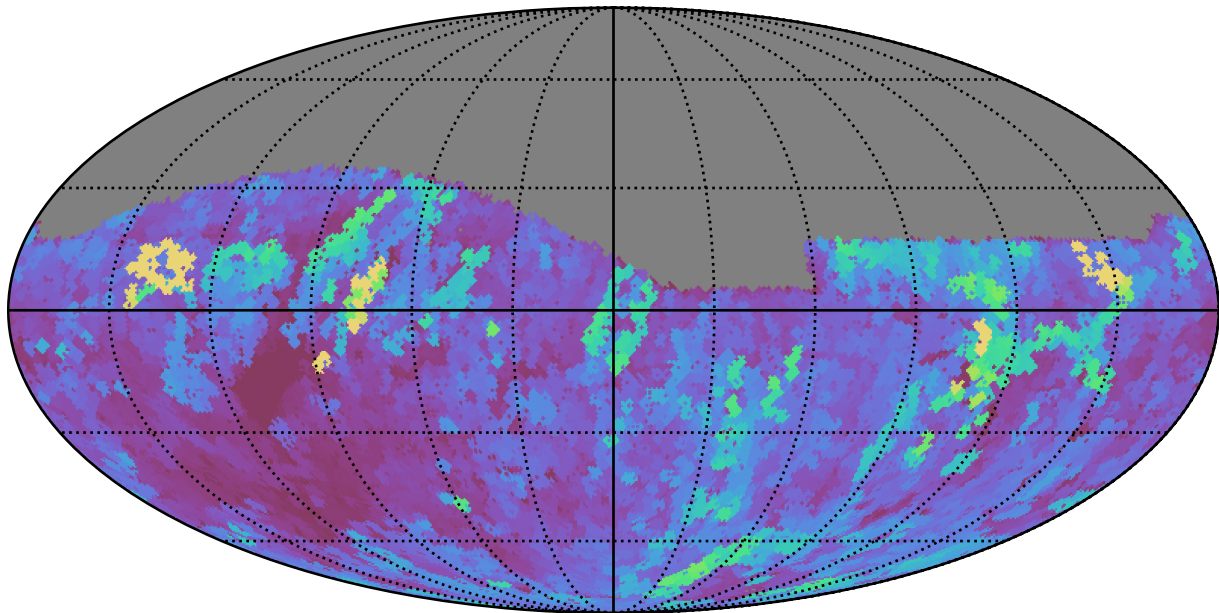
weather_cloudso16v3.4_10yrs Yr 1 r band: Max seeingEff
