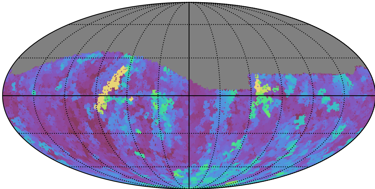
weather_cloudso16v3.4_10yrs Yr 1 g band: Max seeingEff
