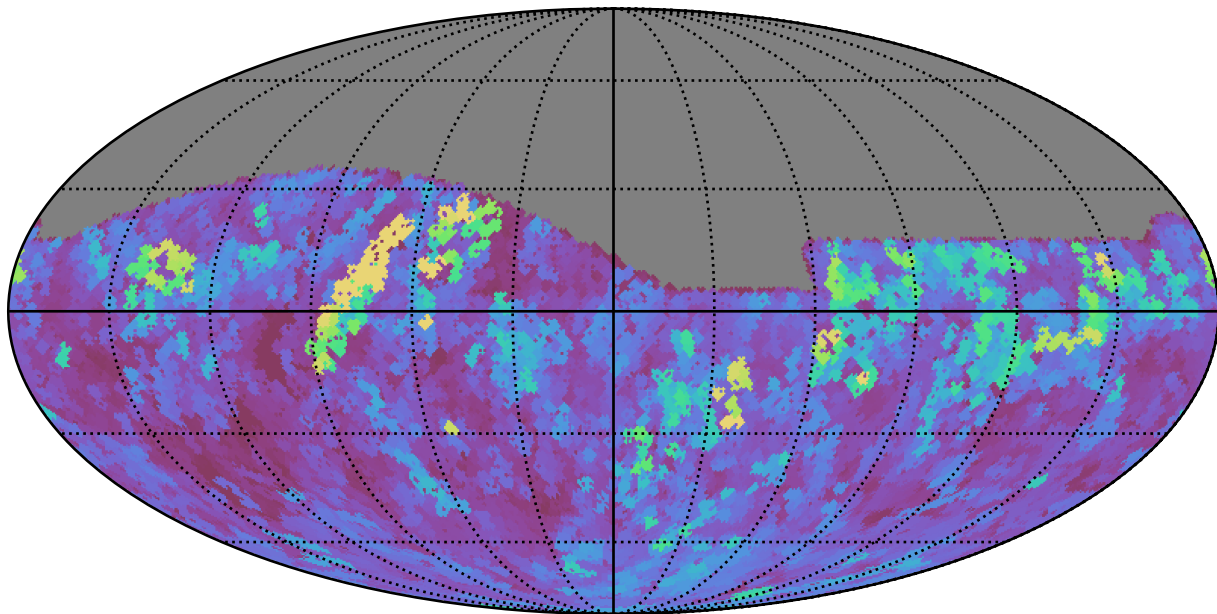
weather_cloudso16v3.4_10yrs Yr 1 all bands: Max seeingEff
