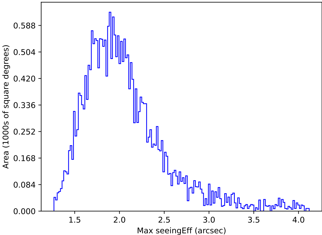
weather_cloudso16v3.4_10yrs Yr 1 all bands: Max seeingEff
