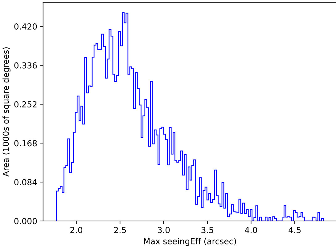
weather_cloudso16v3.4_10yrs WFD y band: Max seeingEff
