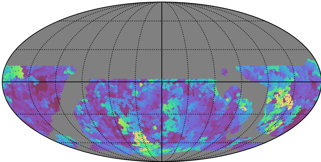
weather_cloudso16v3.4_10yrs WFD u band: Max seeingEff
