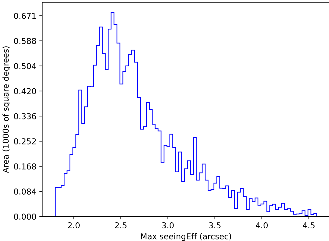
weather_cloudso16v3.4_10yrs WFD u band: Max seeingEff
