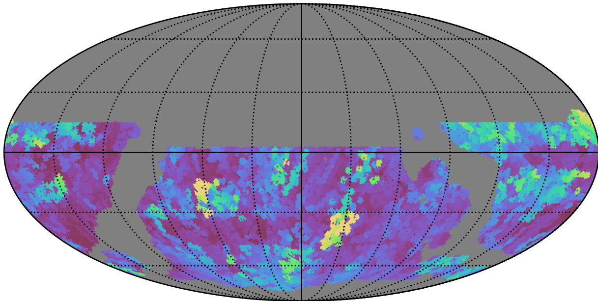
weather_cloudso16v3.4_10yrs WFD r band: Max seeingEff
