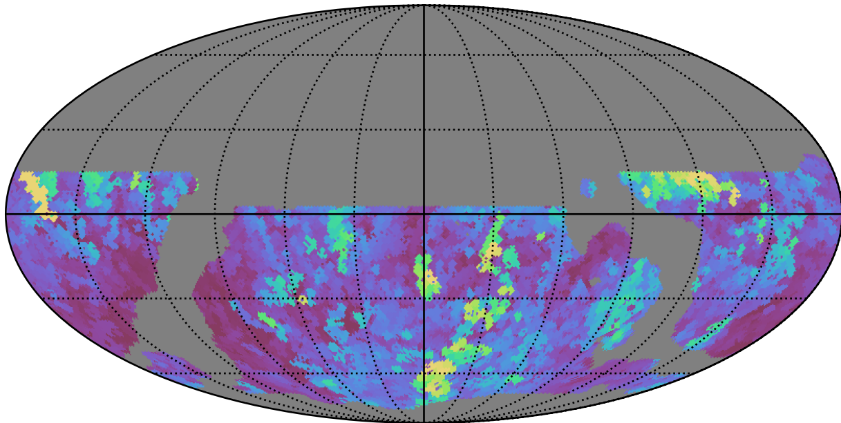
weather_cloudso16v3.4_10yrs WFD i band: Max seeingEff
